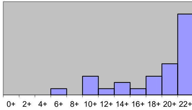
Problem #5 Scores
