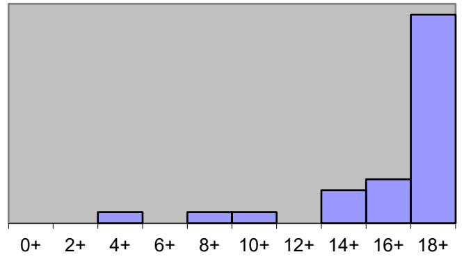
Problem #4 Scores
