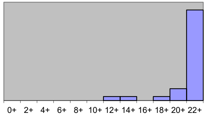
Problem #2 Scores
