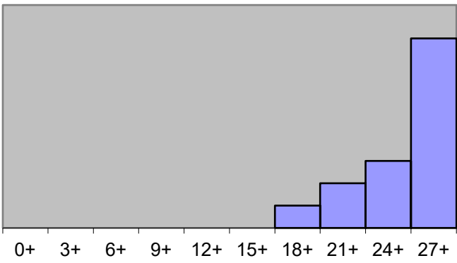
Problem #1 Scores
