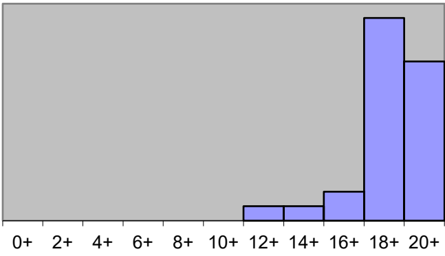
Problem #3 Scores
