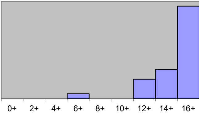
Problem #3 Scores
