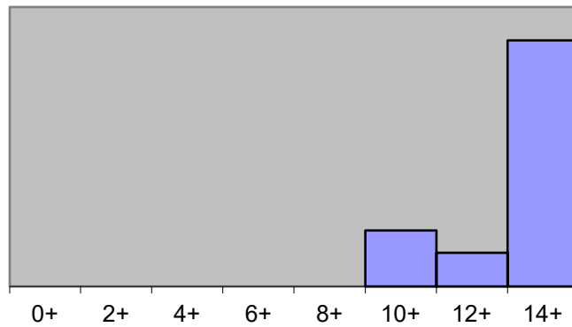
Problem #7 Scores
