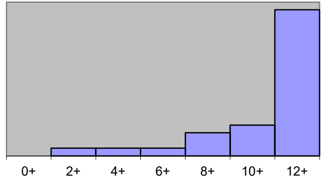
Problem #4 Scores
